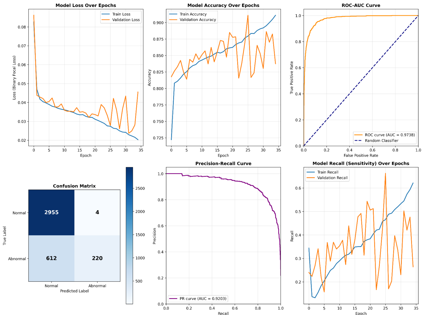
Figure 4-8 Training Convergence and Performance for Model 02 (FL)
